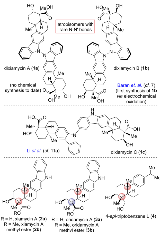
Fig. 1 Indolosesquiterpene alkaloids 1–3 .
