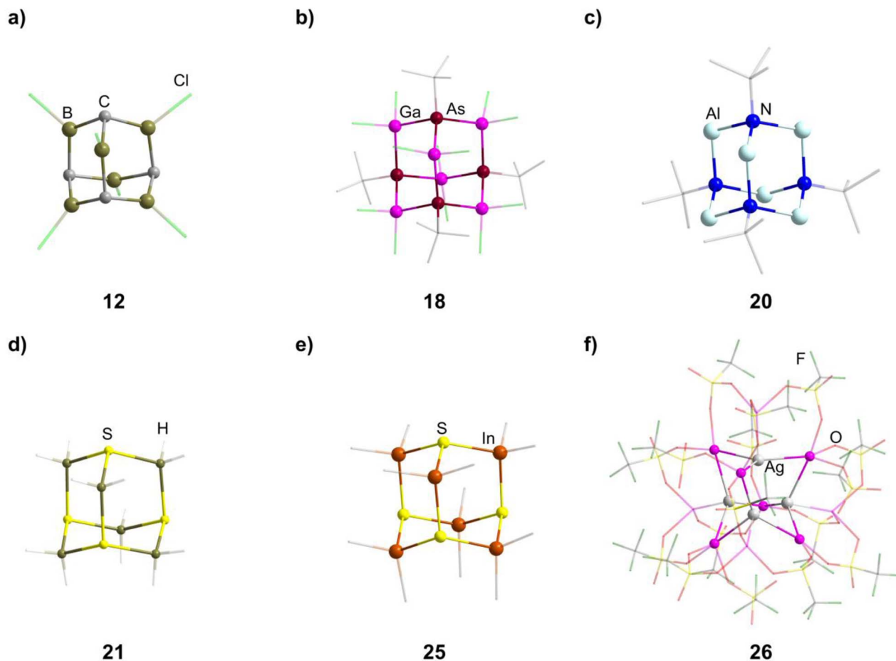
Fig. 2 Examples of adamantane-type compounds with group 13 atoms in the E position: [(CH)_4(BCl)_6] ( 12 , top left (a)), [Li(thf)_4]_2[Li(BuAs)_4(GaCl_2)_6] ( 18 , top center (b)), [Li(thf)_4]_2[Li(BuAl)_4(GaCl_2)_6] ( 20 , top right (c)), Na_2[S_4(BH_2)_6] ( 21 , bottom left (d)), DMPyr_2[S_4(InMe_2)_6] ( 25 , bottom center (e)) and [Ga(C_6H_5Me)_2]_2[AgGa(OTf)_3]_4Ga_6(OTf)_4 ( 26 , bottom right (f)). Hydrogen atoms in the organic ligands and counterions, if present, are omitted for clarity.
