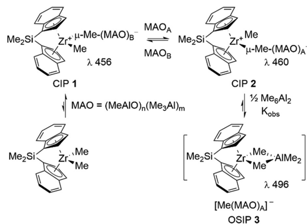
Scheme 1 Activation of \text{SBIZrMe}_2 by MAO. K_{\text{obs}} varies from 2.4 to 6.5 \text{M}^{-1/2} between Al:Zr = 100:1 to 1000:1. 5
