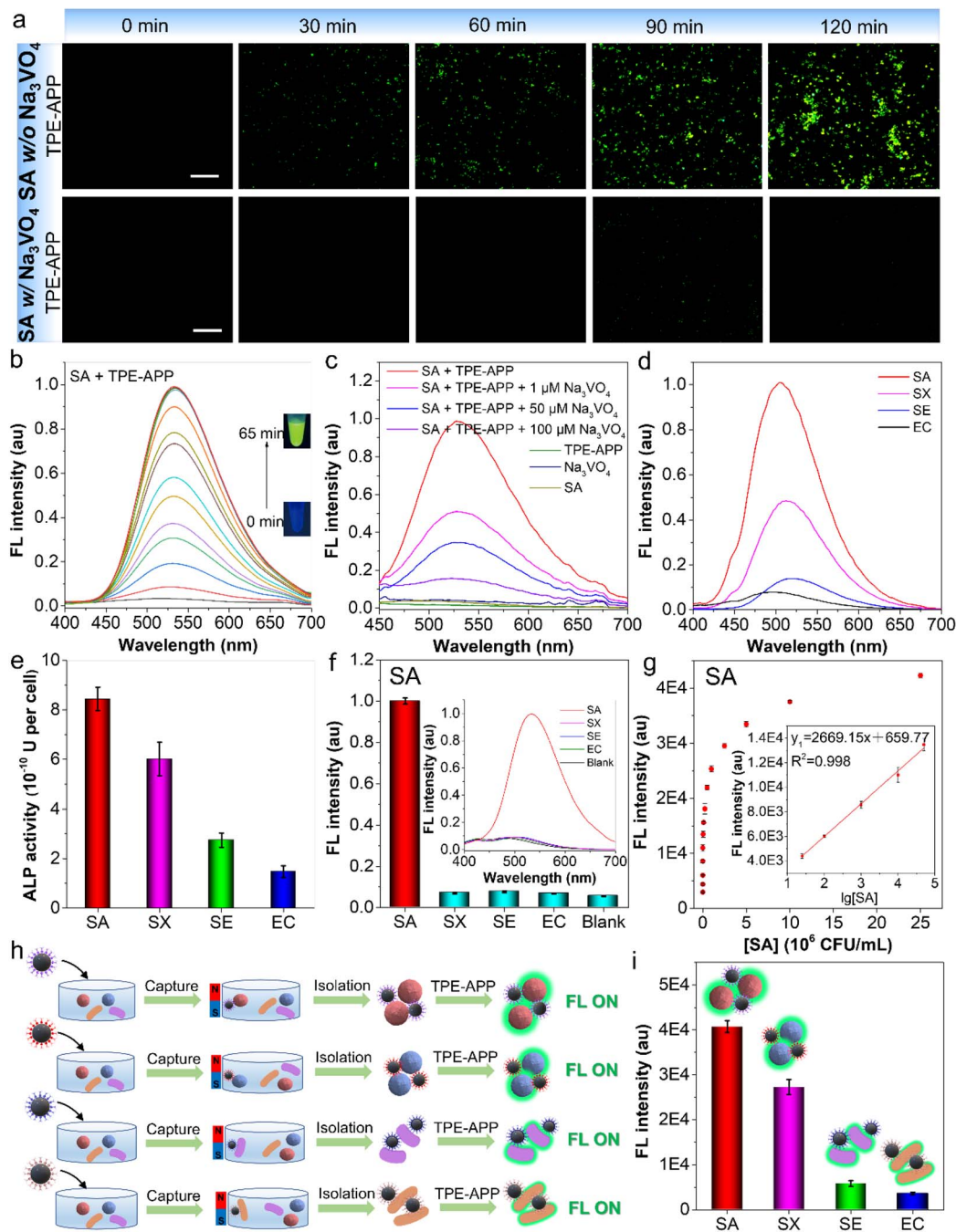
Fig. 2 MNs@phage for target bacterial capture and intracellular ALP response toward the TPE-APP probe for multiple bacterial detection. (a) FL imaging of SA ( 5 \times 10^7 CFU \text{mL}^{-1} ) without (w/o) sodium orthovanadate ( \text{Na}_3\text{VO}_4 ) for 60 min, SA with (w/) \text{Na}_3\text{VO}_4 (100 \mu\text{M} ) for 60 min, followed by incubation with TPE-APP (120 \mu\text{M} ) for 0, 30, 60, 90 and 120 min. Scale bar: 10 \mu\text{m} . (b) FL spectra of SA ( 1 \times 10^8 CFU \text{mL}^{-1} ) incubated with TPE-APP (120 \mu\text{M} ) at different time points. (c) FL spectra of SA in the presence and absence of the TPE-APP probe or \text{Na}_3\text{VO}_4 . (d) FL spectra of SA, SX, SE and EC ( 5 \times 10^7 CFU \text{mL}^{-1} ) incubated with TPE-APP probes (120 \mu\text{M} ) for 2 h, respectively. (e) Monitoring ALP activities in SA, SX, SE and EC. (f) Specificity analysis of the assay for SA detection. The concentration of bacteria was 5 \times 10^6 CFU \text{mL}^{-1} , while the concentrations of the negative control bacteria were 10 times higher than that of the target bacteria. (g) Sensitivity analysis of the assay for SA detection. FL intensity is plotted against SA concentration, with the linear detection range shown in the inset. (h) Schematic illustration of the detection process for four types of bacteria. (i) Detection of four types of bacteria in mixed bacterial samples.
