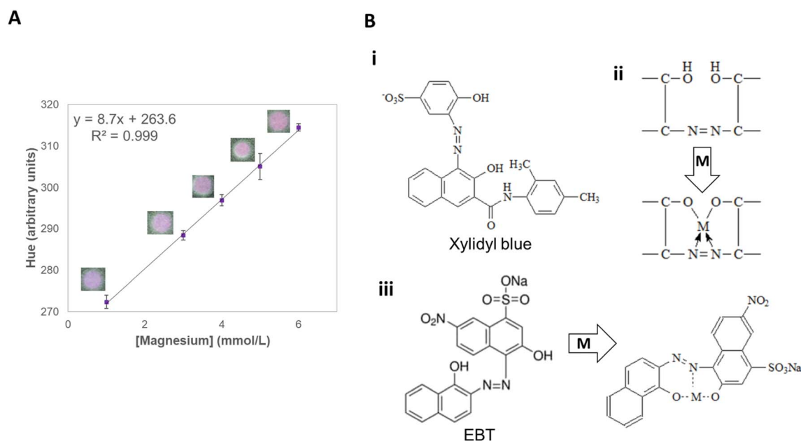
Fig. 4 Detection of magnesium in the proposed \mu PAD. (A) Calibration curve obtained for \text{Mg}^{2+} in concentrations ranging from 1.0 to 6.0 \text{mmol L}^{-1} . (B) Structure of (i) Xylidyl blue before the interaction with the analyte; (ii) the region of Xylidyl blue responsible for binding to \text{Mg}^{2+} before and after the interaction; and (iii) EBT before and after binding to \text{Mg}^{2+} .
