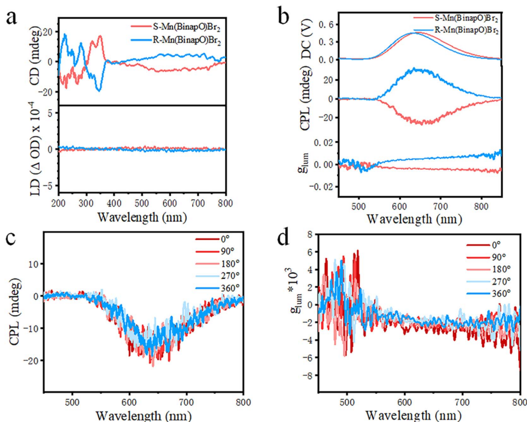
Fig. 2 (a) Circular dichroism absorption (CD) spectrum and linear dichroism absorption (LD) spectrum of R/S -Mn(Binapo)Br 2 . (b) Circularly polarized luminescence (CPL) spectra of R/S -Mn(Binapo)Br 2 with DC, CPL emission and g lum . (c) CPL spectra of S -Mn(Binapo)Br 2 recorded by rotating the sample from 0° to 360°. (d) Variation of g lum of S -Mn(Binapo)Br 2 measured after sample rotation from 0° to 360°.
