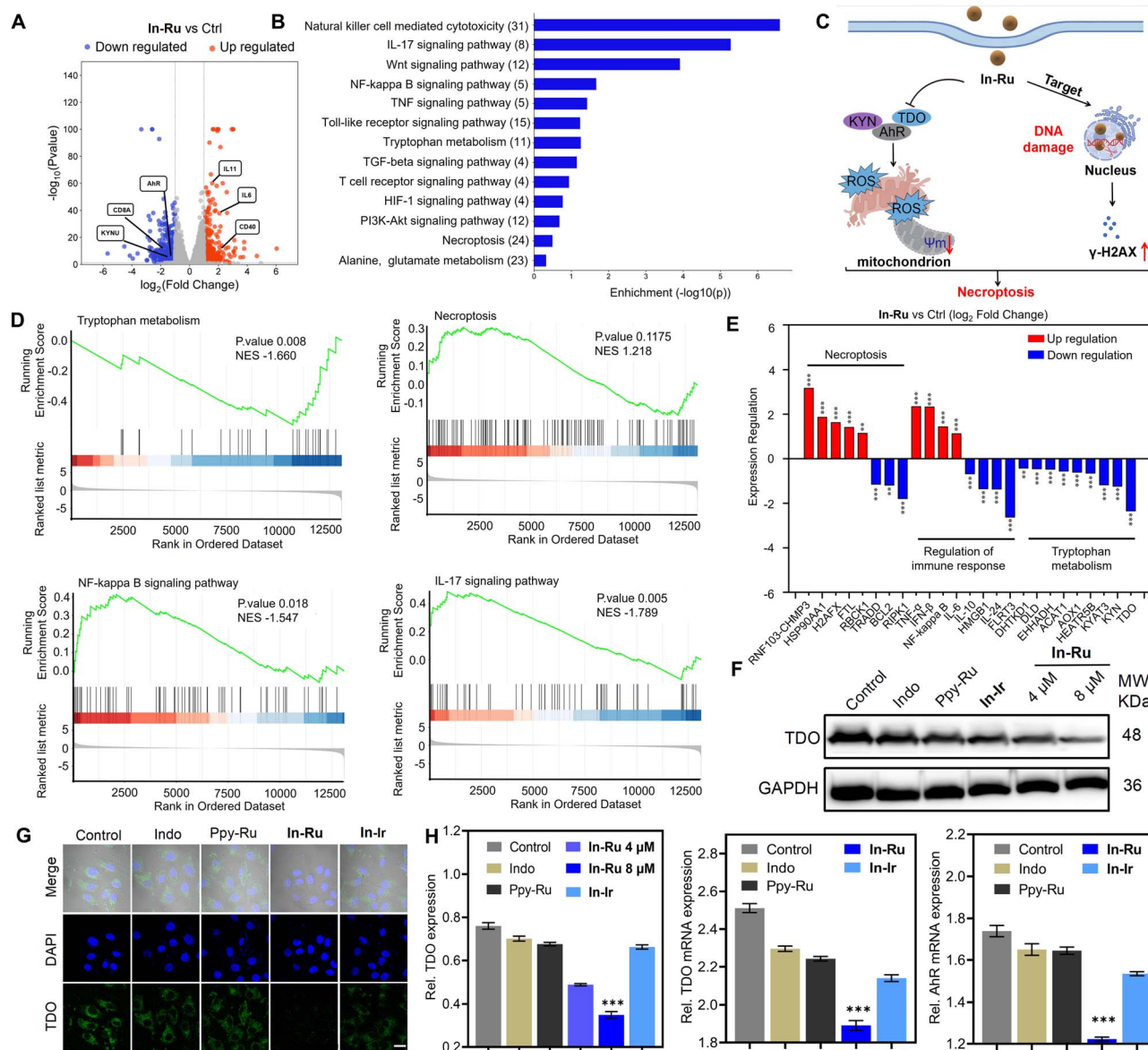
Fig. 4 Assessment of TDO inhibition and ICD-induced immune activation. (A) Volcano plot showing the DEGs in HepG2 cells treated with In-Ru (4 \mu M) for 24 h. Standard: |\log_2FC| > 1 ; q -value < 0.05 . (B) KEGG enrichment analysis of differentially expressed genes after treated by In-Ru (4 \mu M) for 24 h. (C) In-Ru molecule targets the cell nucleus, inducing DNA damage while simultaneously suppressing the expression of TDO. These combined effects lead to necroptosis in HepG2 cells. (D) GSEA reveals negative and positive enrichment of altered genes in cellular processes after treated by In-Ru (4 \mu M) for 24 h. Standard: observed genes > 2 , fold change > 2 and FDR < 0.05 (Tryptophan metabolism, Necroptosis, NF- \kappa B signaling pathway, IL-17 signaling pathway). (E) Expression level changes of the impacted genes involved in necroptosis, regulation of immune response and tryptophan metabolism in HepG2 cells treated with In-Ru. (F) Western blot analysis of TDO inhibition in HepG2 cells treated with various compounds for 24 h. (G) Confocal images of TDO signal in HepG2 cells treated with various compounds for 24 h. FITC: \lambda_{ex} = 488 nm, \lambda_{em} = 525 \pm 20 nm; DAPI: \lambda_{ex} = 364 nm, \lambda_{em} = 454 \pm 20 nm. Scale bar: 20 \mu m. (H) Quantitative analysis for expressions of TDO proteins in (F); statistical analysis of TDO and AhR mRNA expression changes following treatment with various compounds. Error bars: S.D., n = 3 . * p < 0.05 , ** p < 0.01 , *** p < 0.001 , **** p < 0.0001 .
