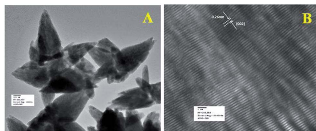
Fig. 5 (a) TEM and (b) HRTEM images of ZnO nanoparticles. HRTEM image was used to calculate the fringe spacing.
