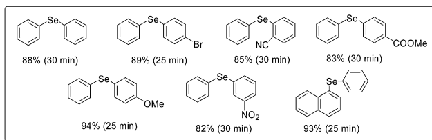
Scheme 16 Zinc mediated microwave-accelerated synthesis of diaryl selenides.
