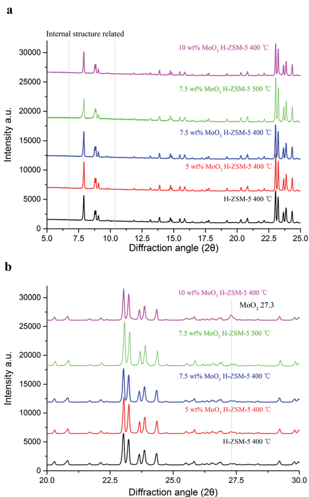
Fig. 2 (a) X-ray diffraction patterns ( 2\theta = 5\text{--}25^\circ ) of \text{MoO}_3/\text{ZSM-5} samples with various \text{MoO}_3 loadings and prepared at 400 °C/500 °C. (b) X-ray diffraction patterns ( 2\theta = 20\text{--}30^\circ ) of \text{MoO}_3/\text{ZSM-5} samples with various \text{MoO}_3 loadings and prepared at 400 °C/500 °C.
