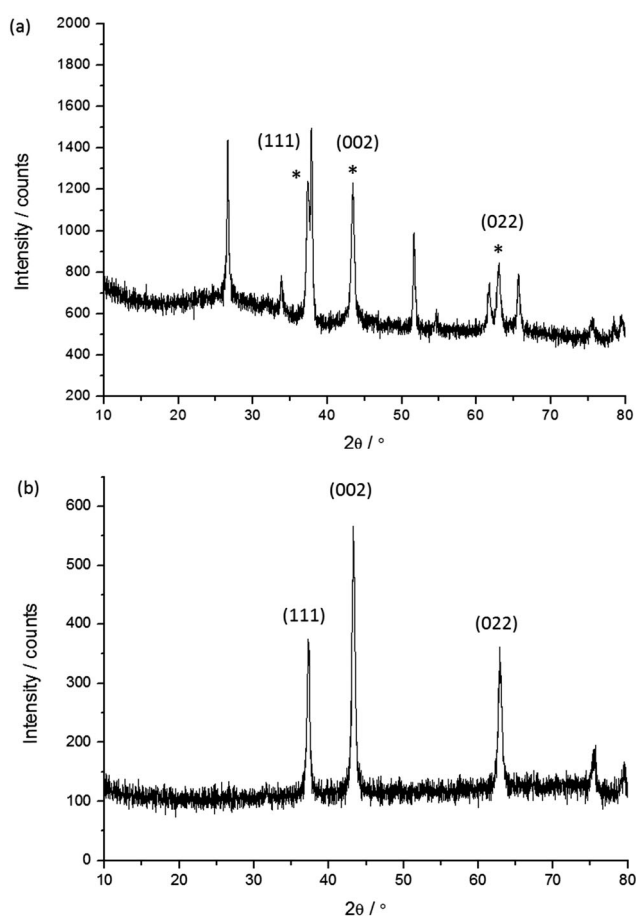
Fig. 5 Representative X-ray diffraction patterns for sample 4 : (a) the NiO film on FTO; (b) the NiO nanoparticles removed from the film. The diffraction peaks indexed with the ( hkl ) notation correspond to the main NiO phase. 25 * Denotes the peaks corresponding to NiO.
