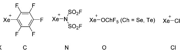
Fig. 106 Examples of Xe-X bonds ( \text{X} = \text{C}, \text{Cl}, \text{N}, \text{O} ) in cations.
