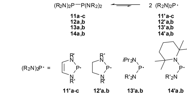
Scheme 13 P–P bond dissociation equilibria for tetraamino-diphosphines ( R' = t\text{Bu} ( 11a ), 2,6- \text{Me}_2\text{C}_6\text{H}_3 ( 11b ), 2,6- \text{iPr}_2\text{C}_6\text{H}_3 ( 11b , 12a ), 2- \text{tBu}_2\text{C}_6\text{H}_4 ( 12b ), \text{iPr} ( 13a , 14b ), \text{SiMe}_3 ( 13b ), \text{Et} ( 14a )).
