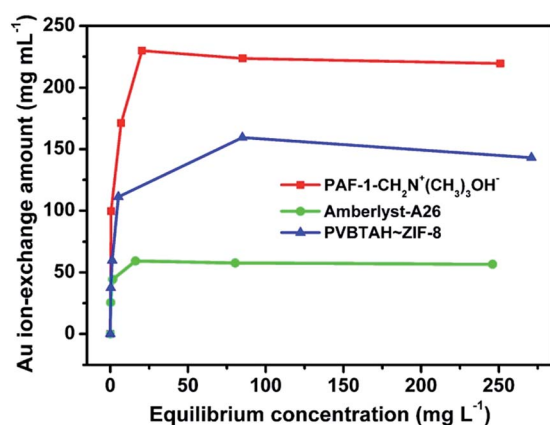
Fig. 3 Volumetric Au(I) adsorption isotherms for PAF-1- \text{CH}_2\text{N}^+(\text{CH}_3)_3\text{OH}^- , Amberlyst-A26 and PVBTAAH-ZIF-8.
