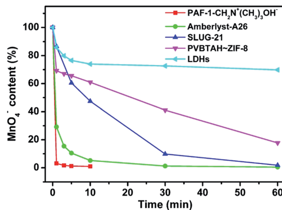
Fig. 4 Comparison of the ion exchange performances of PAF-1- \text{CH}_2\text{N}^+(\text{CH}_3)_3\text{OH}^- and other ion exchange materials in removing model \text{MnO}_4^- ions.
