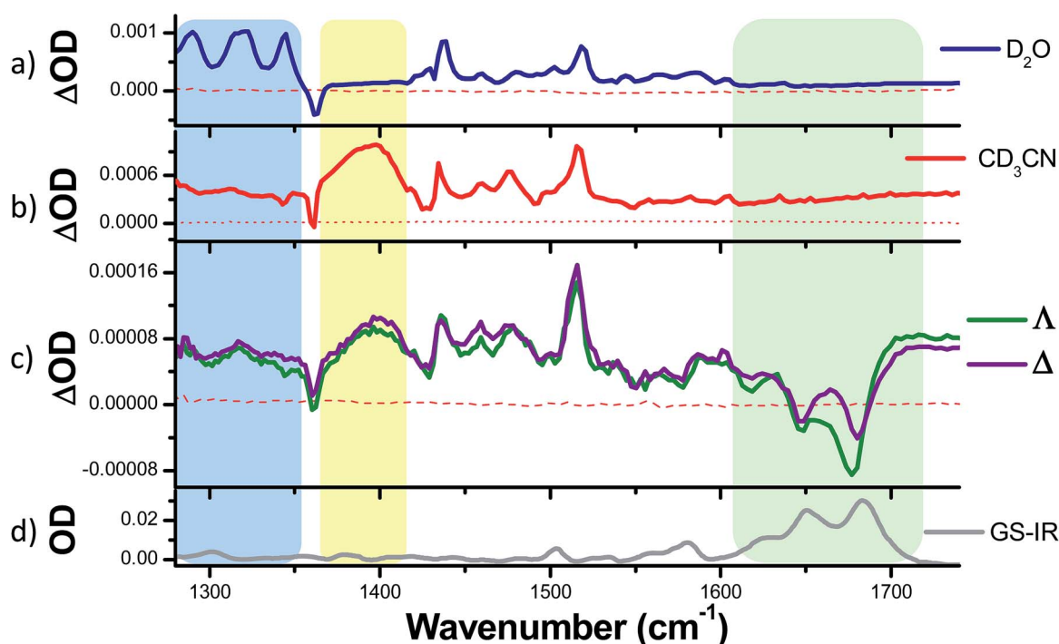
Fig. 8 TRIR spectra recorded 35 ps after 400 nm excitation of (a) 1 \cdot 2\text{Cl}^- (500 \mu\text{M} ) in \text{D}_2\text{O} , (b) 1 \cdot 2\text{PF}_6^- (500 \mu\text{M} ) in \text{CD}_3\text{CN} and (c) \Delta - and \Lambda -[ 1 ] 2\text{Cl}^- (400 \mu\text{M} ) and a duplex DNA oligonucleotide \text{d}(\text{TCGGCGCCGA})_2 (500 \mu\text{M} duplex) and (d) FTIR spectrum of oligonucleotide \text{d}(\text{TCGGCGCCGA})_2 (500 \mu\text{M} duplex) in deuterated potassium phosphate buffer (50 mM) pH 7. The blue and yellow coloured regions highlight the characteristic transient bands for the excited state of 1 , while the green coloured region highlights the bands associated with the DNA base pairs.
