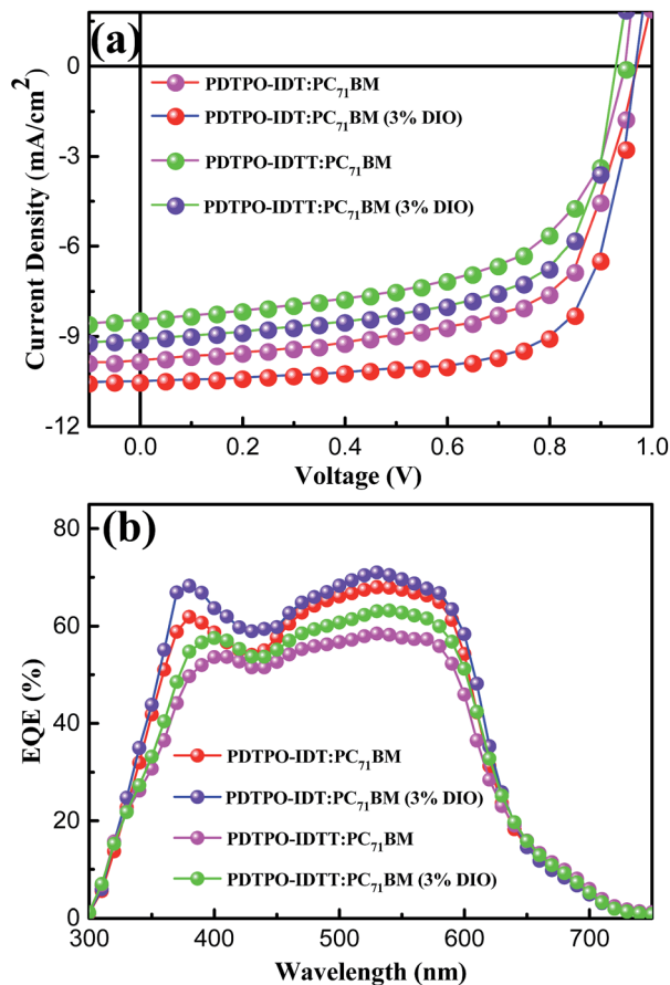
Fig. 4 (a) J - V characteristics curves of PDTP0-IDT : PC 71 BM (1 : 2, w/w) and PDTP0-IDTT : PC 71 BM (1 : 2, w/w) based PSCs without or with 3% DIO (v/v) under AM 1.5 G at 100 \text{ mW cm}^{-2} . (b) Corresponding EQE spectra of PDTP0-IDT : PC 71 BM and PDTP0-IDTT : PC 71 BM based PSCs without or with 3% DIO (v/v).
