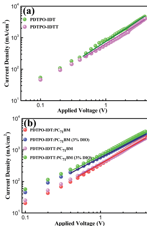
Fig. 5 Current-voltage ( I - V ) characteristics of pure films (a) and blend films (b) (with or without 3% DIO) PDTP0-IDT : PC 71 BM (1 : 2, w/w) and PDTP0-IDTT : PC 71 BM (1 : 2, w/w) in space-charge-limited current (SCLC) devices.
