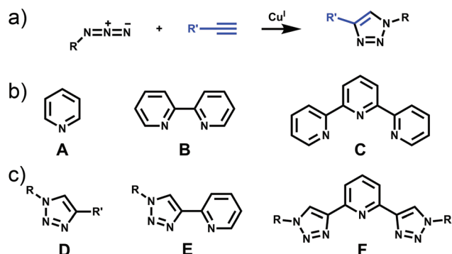
Fig. 2 (a) The copper(I) catalysed ‘click’ reaction between an azide and alkyne generating 1,4-disubstituted-1,2,3-triazoles; (b) pyridyl-based chelating units (A–C) and (c) related 1,2,3-triazoles ligands (D–F).
