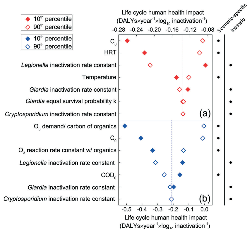
Fig. 5 The top seven input parameters to which human health impacts are most sensitive, for chlorination (a) and microplasma ozonation (b), expressed in \text{DALYs} \times \text{year}^{-1} \times \log_{10} \text{pathogen inactivated}^{-1} . Sensitivity analysis for the rest of the parameters can be found in Fig. S4a and b in the ESI.†
