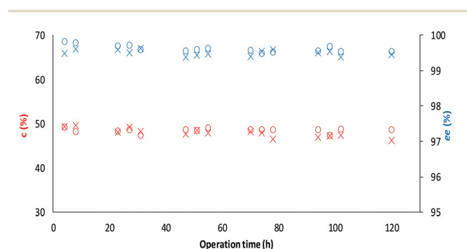
Fig. 8 Long term stability of the CaLB entrapped in the TDP sol-gel system in KR of the alcohol rac-1a ( c %; x, ee_{(R)-2a} %; o) and amine rac-3a ( c %; o, ee_{(R)-4a} %; x) in a continuous-flow reactor (60 °C, flow-rate of 0.1 mL min -1 ).
