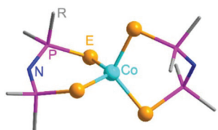
Fig. 1 Molecular structure diagram of \text{Co}([\text{EPR}_2]_2\text{N})_2 ( \text{E} = \text{S}, \text{Se}, \text{Te} ; \text{R} = \text{Ph}, \text{tPr} ). The hydrogen atoms and the R groups are not shown for clarity.
