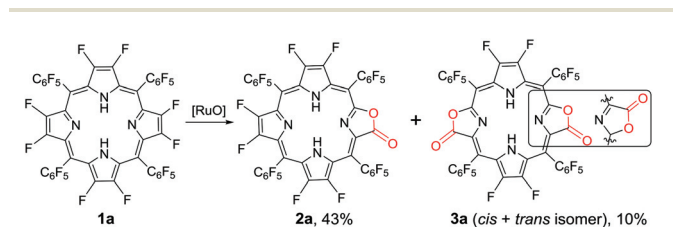
Scheme 1 Oxidation of 1a by the “RuCl 3 + Oxone®” protocol. Conditions: 1a 0.05 mmol, RuCl 3 · n H 2 O 0.01 mmol, 2,2′-bipyridine 0.01 mmol, Oxone® 1 mmol, NaOH 1 mmol, 1,2-dichloroethane/H 2 O = 1/1 (v/v) 60 mL, 80 °C, 1 h. See the ESI† for details.
