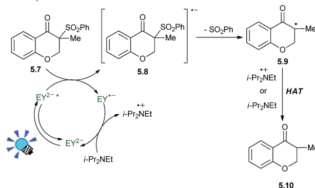
Scheme 5 Reductive desulfonation of ketosulfones.
