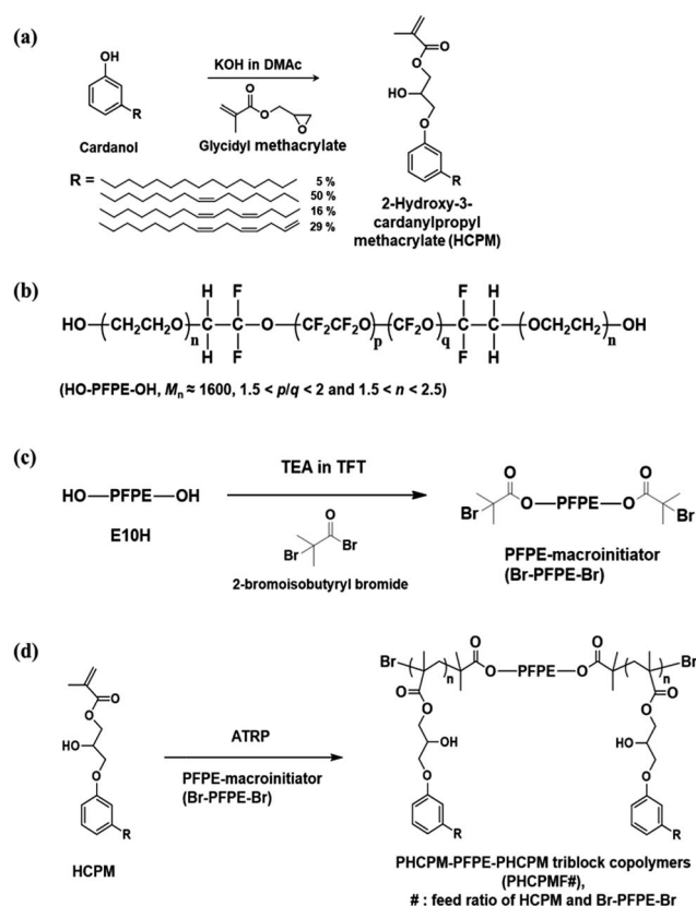
Fig. 1 (a) Synthesis of 2-hydroxy-3-cardanylpropyl methacrylate (HCPM). (b) Chemical structure of E10H. Synthesis of (c) PFPE-macroinitiator (Br-PFPE-Br) and (d) PHCPMF-triblock copolymers (PHCPMF#).
