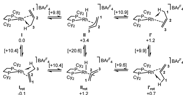
Scheme 10 Computed mechanisms for fluxionality and D-label scrambling in [\text{1-(propene)}][\text{BAR}^{\text{F}}_4] in the solid-state. Gibbs free energies are indicated in \text{kcal mol}^{-1} with those for transition states provided in square brackets.
