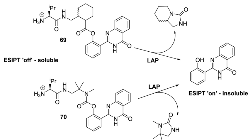
Scheme 66 Leucine-functionalised HPQ fluorescent probes 69 and 70 that were developed to allow for the rapid and selective detection of LAP. Measurement conditions: pH = 7.5.
