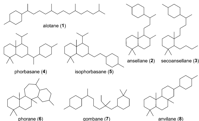
Fig. 2 Alotane (1) and its proposed sesterterpenoid skeletal derivatives.
