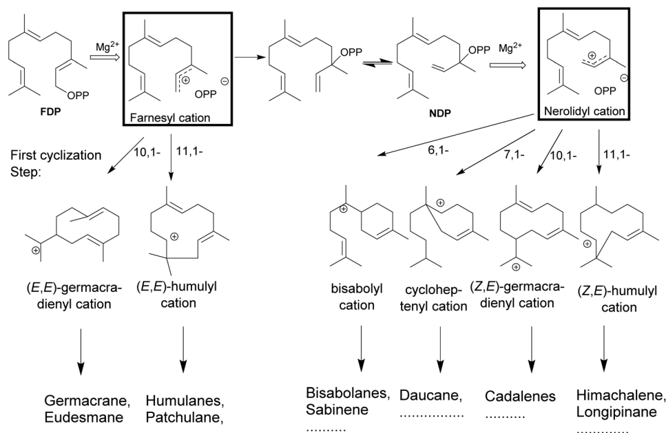
Fig. 3 Possible cyclizations of (2E,6E) - or (2Z,6E) -farnesyl cations and some resulting carbon skeletons of sesquiterpenes. The loss of the diphosphate anion initiates the formation of a highly reactive transoid farnesyl cation, which after isomerization undergoes various cyclizations and rearrangements, methyl- or hydride shifts. Due to its constrained geometry, the electrophilic transoid farnesyl cation can attack only the distant C10–C11 double bond. However, the C2–C3 double bond isomerization to (2Z,6E) -farnesyl cations, the geometrically suitable conformation leading to other cyclic products.
