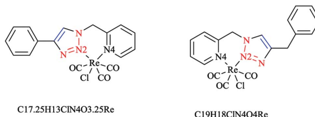
\text{C}_{19}\text{H}_{18}\text{ClN}_4\text{O}_4\text{Re}
