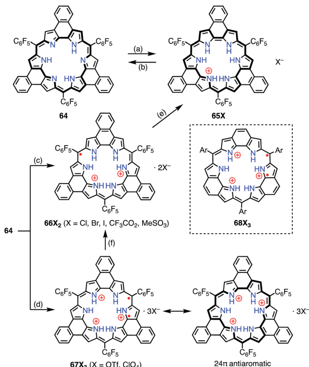
Fig. 21 Protonation-induced formation of the planar rosarin derivatives 64 . (a) Saturated \text{Na}_2\text{S}_2\text{O}_4 (aq), \text{CH}_2\text{Cl}_2 , rt, 30 min, 87%; (b) \text{MnO}_2 or triethylamine; (c) \text{HX} ( \text{X} = \text{Cl}, \text{Br}, \text{I}, \text{CF}_3\text{CO}_2, \text{MeSO}_3 ), \text{CH}_2\text{Cl}_2 , rt; (d) \text{HX} ( \text{X} = \text{OTf}, \text{ClO}_4 ), \text{CH}_2\text{Cl}_2 , rt; (e) \text{Me}_{10}\text{Fc}, \text{HI} ; (f) \text{TBAX} ( \text{X} = \text{Cl}, \text{Br}, \text{I} ), \text{CH}_2\text{Cl}_2 , rt.
