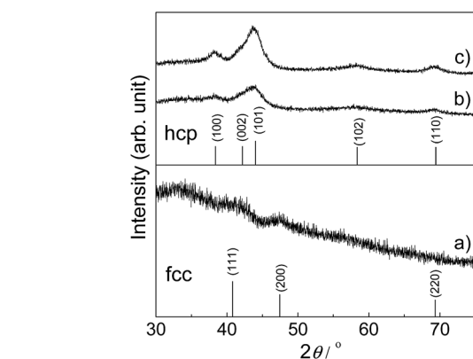
Fig. 2 XRD patterns of Ru-NP samples prepared from (a) 10 wt%, (b) 15 wt% and (c) 20 wt% Ru-deposited Ca(NH 2 ) 2 . JCPDF card numbers are (hcp) 01-070-0274 and (fcc) 01-088-2333.
