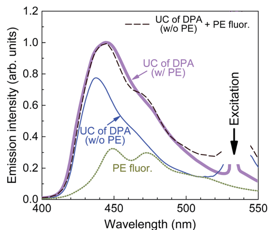
Fig. 6 Fluorescence spectrum (dotted line) of the singlet sink PE in PMMA ( c_{\text{PE}} = 0.01 wt%), UC spectra of DPA/PtOEP/PMMA ( c_{\text{DPA}} = 25 wt%, c_{\text{PtOEP}} = 0.01 wt%) without (thin line) and with (thick line) PE ( c_{\text{PE}} = 0.01 wt%), and a sum of the first two spectra (dashed line) at a ratio of 1/3 and 2/3 , respectively.
