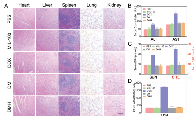
Fig. 9 (A) H&E analyses of the major organs after treatment (scale bar: 100 \mu m). (B) The levels of the serum liver function markers ALT and AST. (C) The levels of the serum kidney function markers BUN and CRE. (D) The serum LDH levels.
