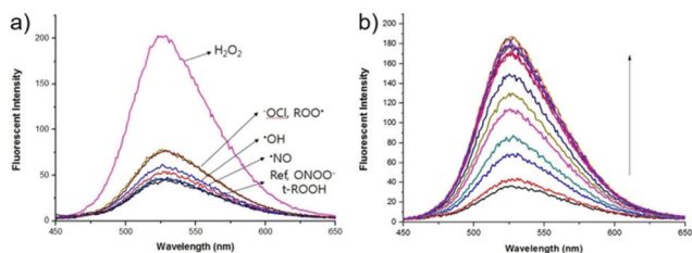
Fig. 66 (a) Fluorescence spectra of probe 45 (2 μM) with various ROS (200 μM) and (b) fluorescence titration of probe 45 (2 μM) upon addition of \text{H}_2\text{O}_2 (0–100 eq.) in PBS (pH 7.4) solution containing 1% DMF after incubation for 2 h at 25 °C at an excitation wavelength of 405 nm, and excitation and emission slit widths of 3 and 5 nm, respectively. Copyright 2015 Nature.
