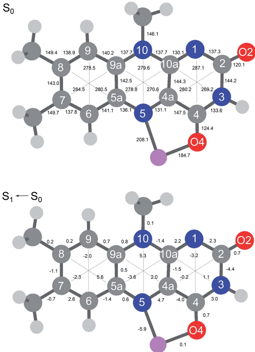
Fig. 6 (Top) Absolute distances (in pm) of Li + LF in its electronic ground state (S 0 ) calculated at the PBE0/cc-pVDZ level. (Bottom) Relative changes in bond distances upon electronic S 1 excitation. Positive (negative) values indicate elongations (contractions). Corresponding data for LF and M + LF with M = Na–Cs are available in Fig. S5 in ESI.†
