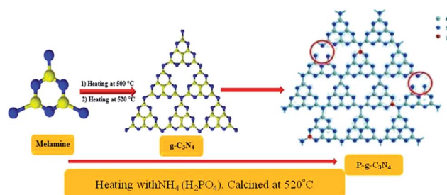
Scheme 2 Synthesis of P-g-C 3 N 4 by the calcination method.
