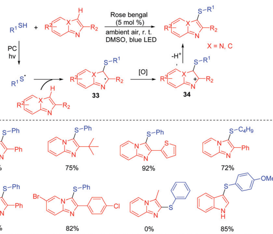
Scheme 16 Regioselective sulfenylation of imidazopyridines.
