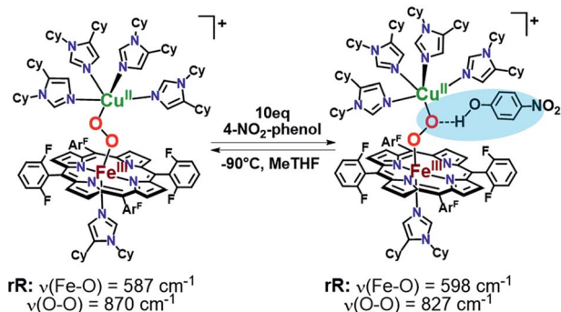
Scheme 2 Previously reported hydrogen-bonded adduct that formed upon addition of 10 equivalents of 4-nitrophenol to a low-spin heme-peroxo-copper complex. Resonance Raman results reported were consistent with the rR in this work (Table 1), where a decrease is observed in the \nu(\text{O-O}) when H-bonding groups interact with the peroxo core.
