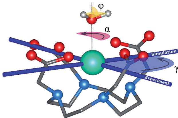
Fig. 1 Main geometrical parameters employed for magneto-structural correlations. \alpha is the angle of rotation around the Dy–O AWM bond; \gamma_{0,1} represents the angles between the calculated and experimental easy-axis of magnetization for the ground and first excited Kramers' doublets; and \phi is the angle between the Dy–O AWM bond and the plane of the water molecule. The dysprosium atom is coloured in light green, oxygen atoms in red, nitrogen atoms in cyan, carbon atoms in grey and hydrogen AWM atoms in white. Hydrogen atoms of DOTA were not reported for the sake of clarity.
