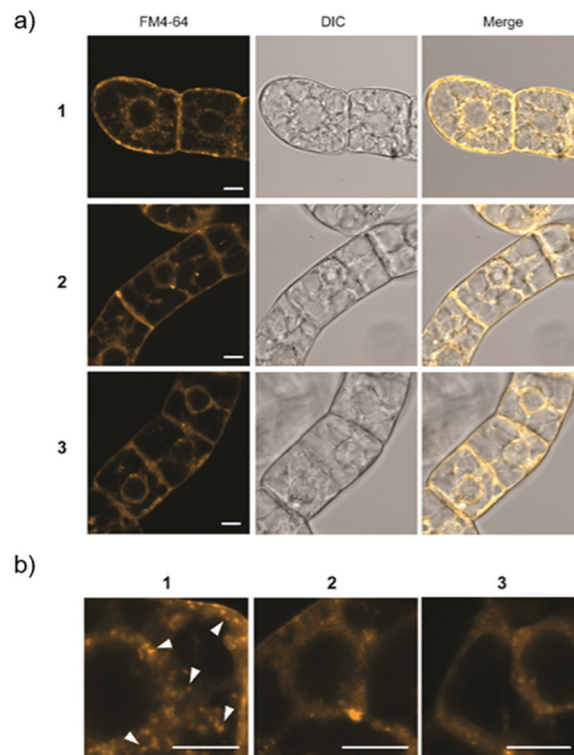
Fig. 3 CSLM imaging of BY-2 cells. (a) Cells treated with each Raman probe were stained with FM4-64 (yellow). (b) Expanded CSLM images for the cells treated with 1 , 2 , or 3 . Arrowheads show vesicles with a size less than 500 \text{ nm} induced by internalization of 1 . Scale bars are 10 \mu\text{m} .
