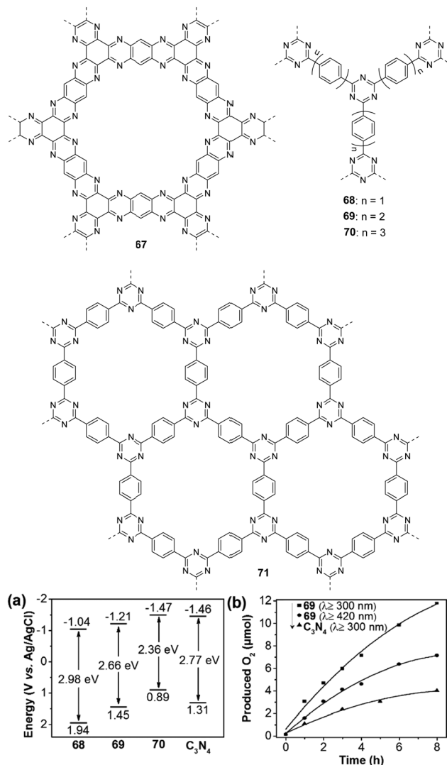
Fig. 16 Chemical structures of polymers 67–71 ; (a) band structure diagram and (b) time course of the O_2 production for polymer 69 and C_3N_4 . Reprinted with permission from ref. 164. Copyright 2018 Wiley-VCH.
