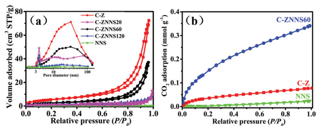
Fig. 3 (a) \text{N}_2 adsorption-desorption isotherms and pore size distribution curves (inset) of C-Z, NNS, C-ZNNS20, C-ZNNS60, and C-ZNNS120. (b) \text{CO}_2 adsorption isotherms of NNS, C-Z, and C-ZNNS60.
