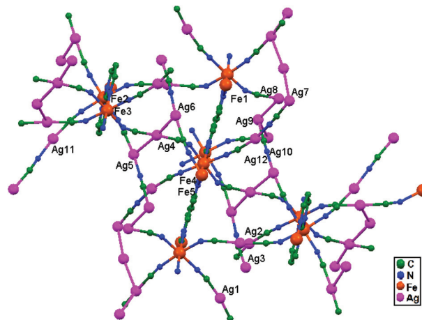
Fig. 56 The coordination environments around crystallographically inequivalent iron and silver atoms and the ligand-unsupported argentophilic interactions in \{\text{Fe}(\text{pmd})\}[\text{Ag}(\text{CN})_2][\text{Ag}_2(\text{CN})_3] , 92 .
