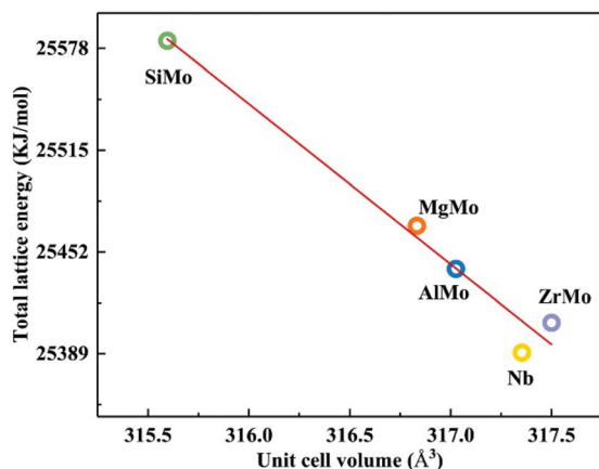
Fig. 34 Correlation between the lattice energy and molecular volume of different \text{NdNbO}_4 -based ceramics (reprinted with permission from ref. 206. Copyright 2019 Elsevier).
