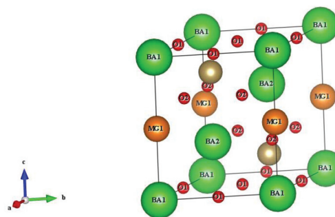
Fig. 35 Crystal structure of a hexagonal \text{Ba}(\text{Mg}_{1/3}\text{Ta}_{2/3})\text{O}_3 system.
