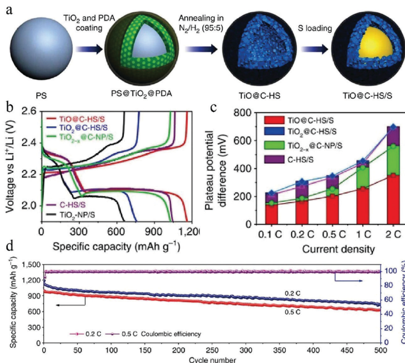
Fig. 16 (a) Schematic illustration of the synthesis process of the \text{TiO}_2@ \text{C-HS/S} composite. (b) Second-cycle galvanostatic charge/discharge voltage profiles at 0.1C. (c) Potential differences between the charge and discharge plateaus at various current densities of the electrodes. (d) Prolonged cycling life and coulombic efficiency of the \text{TiO}_2@ \text{C-HS/S} electrode at 0.2 and 0.5C. Reproduced with permission. 4a Copyright 2016, Nature.
