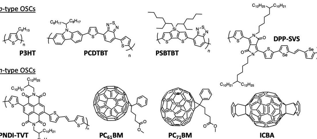
Fig. 5 Chemical structures of P3HT , PCDTBT , PSBTBT , DPP-SVS , PNDI-TV , PC 61 BM , PC 71 BM and ICBA .
