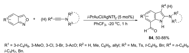
Scheme 73
