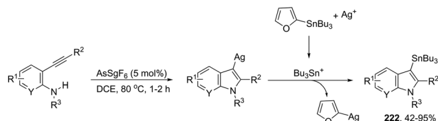
Scheme 260
