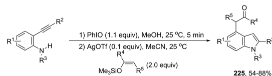
Scheme 263
