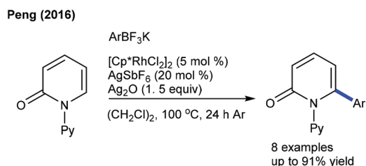
Scheme 7 Arylation of pyridones using aryl trifluoroborates.
