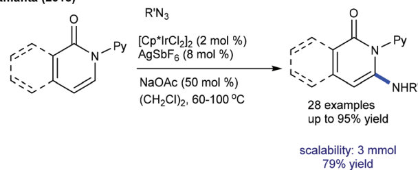
Scheme 147 C3-Amidation of isoquinolones and pyridones with azides.
