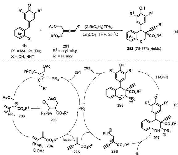
Scheme 64 [4 + 2] annulation of p -QMs with allenoates.
