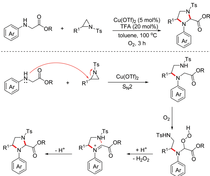
Scheme 10
