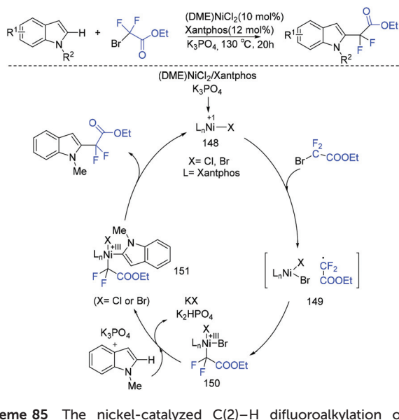
Scheme 85 The nickel-catalyzed C(2)-H difluoroalkylation of C-3 unsubstituted indoles.
